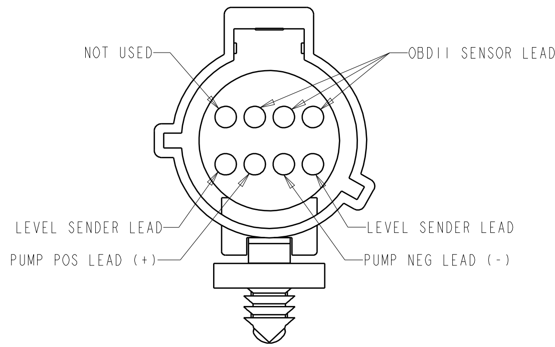
CONNECTOR MODULE MAIN PINOUT DETAIL SCALE 2:1
